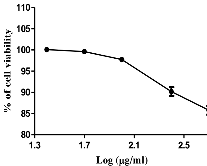
IC50 graph
